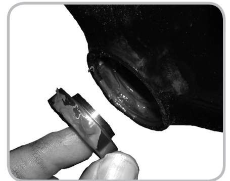
Figure 14.8. Grease on the frame and the non-drive side bearing (with the lip facing in)
