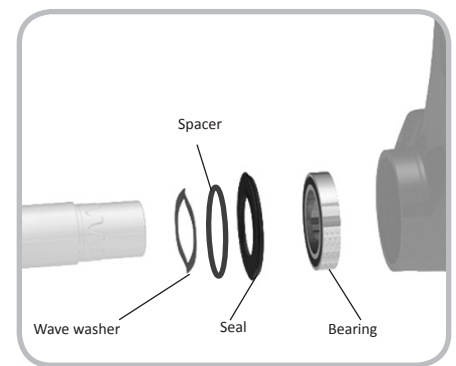
Figure 14.39. SRAM bearing set
