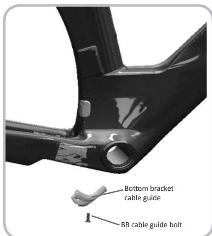
Figure 7.2. Exploded assembly of frame and bottom bracket cable guide
