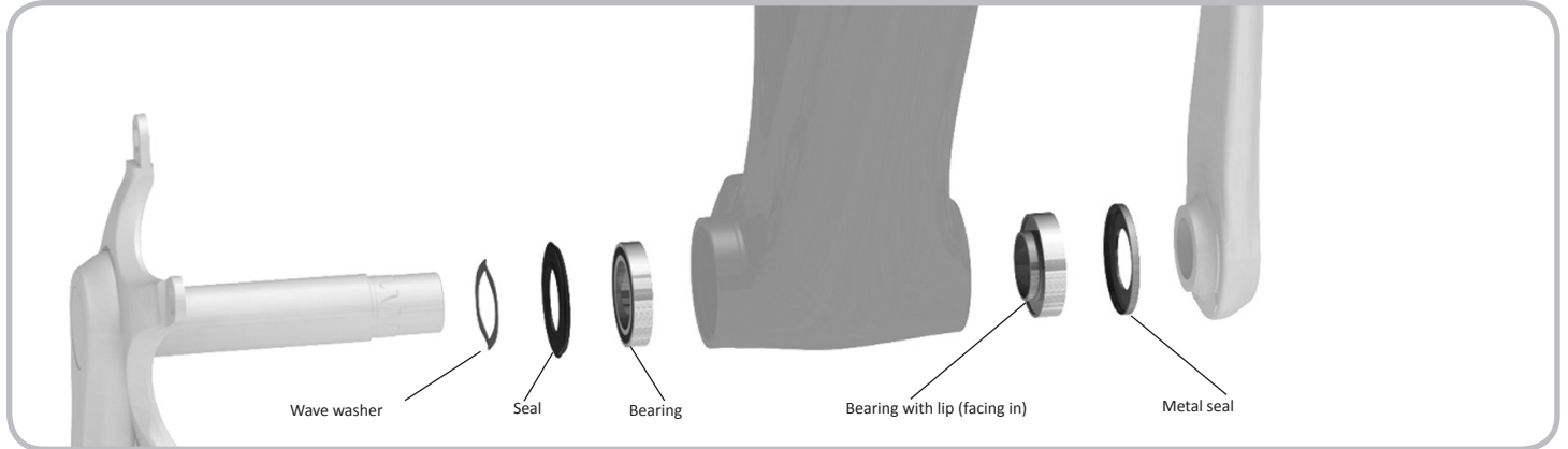
Figure 14.6. SRAM bearing set
