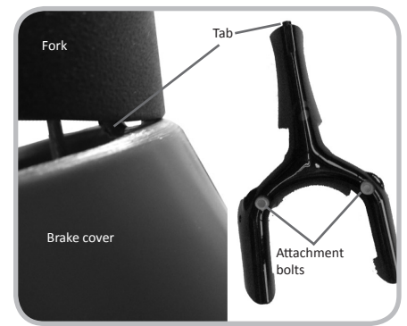
Figure 10.11. Attachment points of front brake cover
