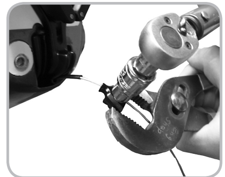
Figure 11.5. Holding the wedge while tightening the cable clamp nut
