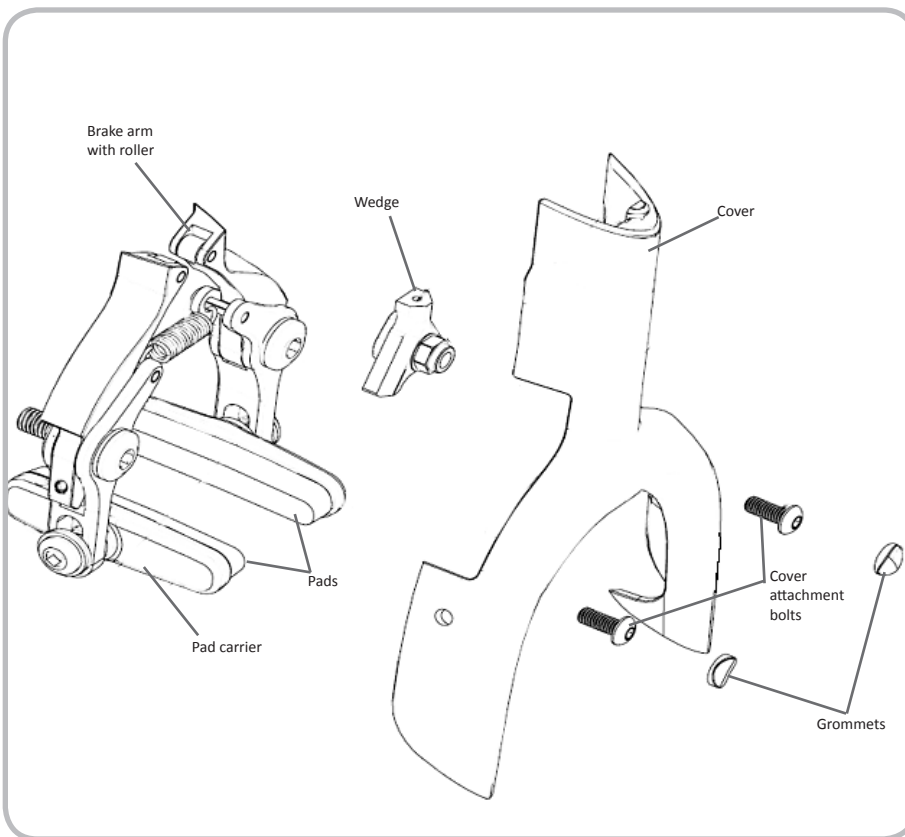
Figure 10.1. Exploded view of front brake
