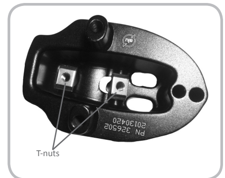
Figure 7.10. Underside of mono-spacer
