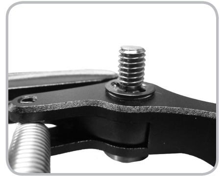
Figure 10.2. E-clip on brake bolt
