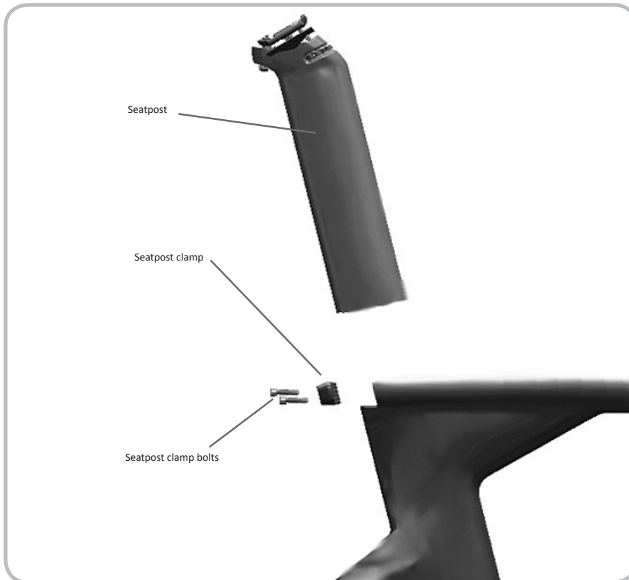
Figure 4.1. Exploded diagram of Speed Concept frame and seatpost
