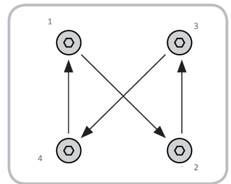
Figure 2.1. Bolt tightening sequence
