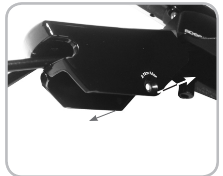
Figure 7.21. Spreading the stem cover
