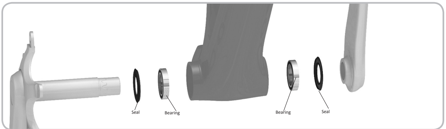
Figure 14.15. Shimano bearing set
