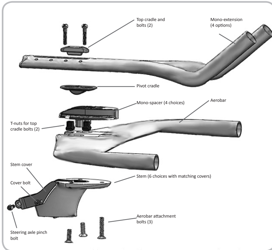
Figure 7.1. Exploded assembly of stem, aerobar, and mono-extension
