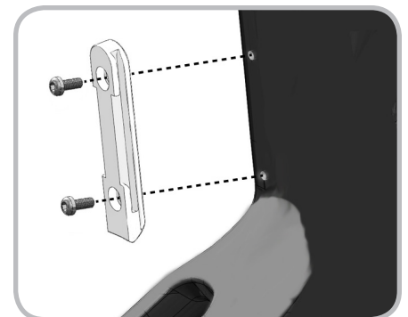
Figure 13.2. Attaching the track to the rear of the seat tube. Note orientation of spring-loaded button.
