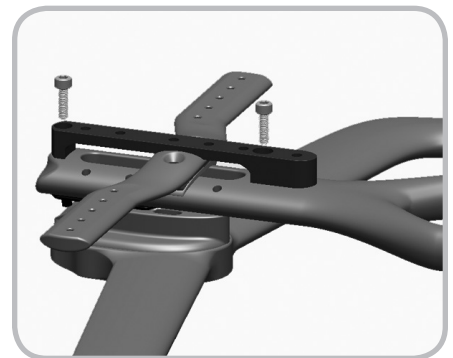
Figure 13.6. The cage mount attaches to the mono-extension
