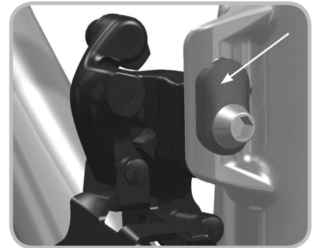
Figure 9.2. Spherical washer for carbon hanger (required)
