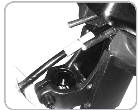
Figure 7.20. Housing window in the top tube
