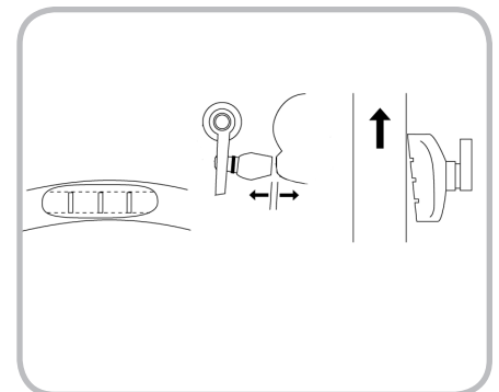
Figure 10.9. Brake pad alignment: carrier aligned with rim, pad face parallel to rim face, slight toe-in
