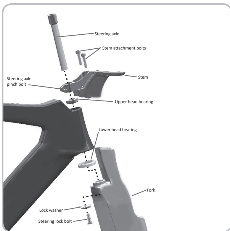
Figure 6.1. Fork attachment exploded diagram
