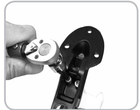
Figure 6.6. Stem-to-fork attachment bolts (two)
