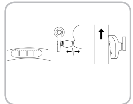
Figure 11.7. Brake pad alignment: carrier aligned with rim, pad face parallel to rim face, slight toe-in
