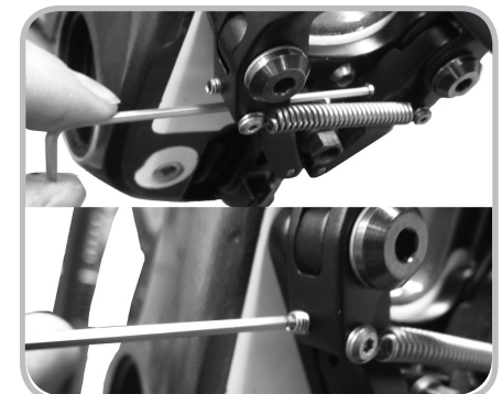
Figure 11.8. Centering the left and right brake pads.
