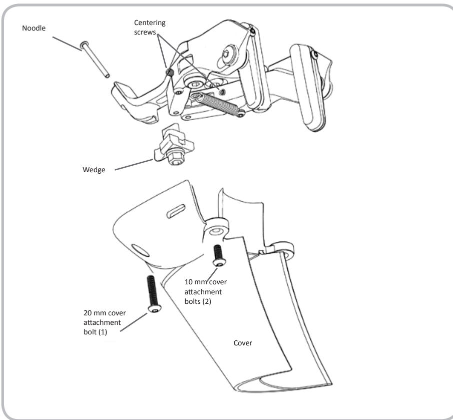
Figure 11.1. Exploded diagram of rear brake
