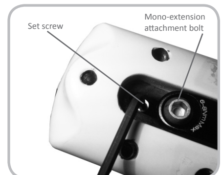
Figure 7.11. Mono-extension bolts allow fore/aft adjustment and control tilt of bar. Set screw prevents movement after adjustment.
