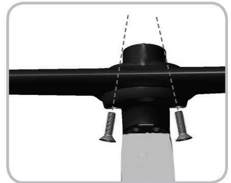
Figure 7.23. Side attachment bolts go in at an angle
