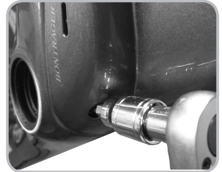
Figure 11.10. Attaching the rear brake cover with front 20 mm bolt
