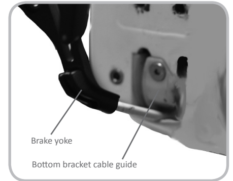
Figure 7.6. Brake yoke with housing connected
