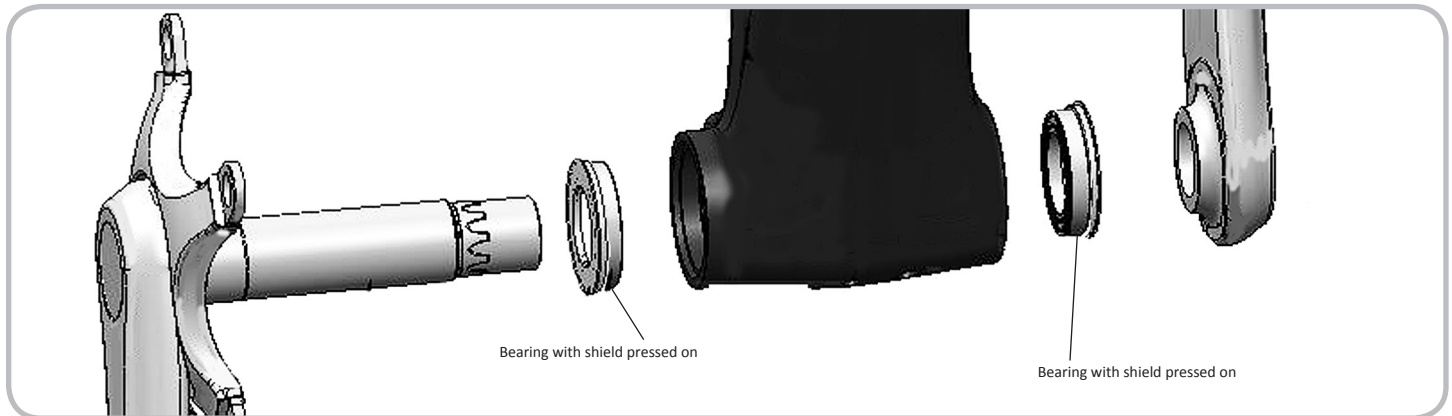
Figure 14.33. FSA bearing set
