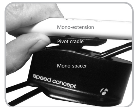
Figure 7.9. Pivot cradle between mono-extension and mono-spacer
