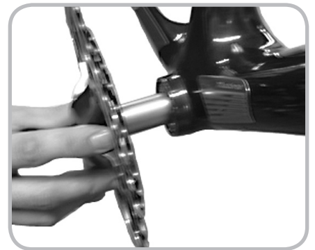
Figure 14.13. Sliding the axle through the bearings
