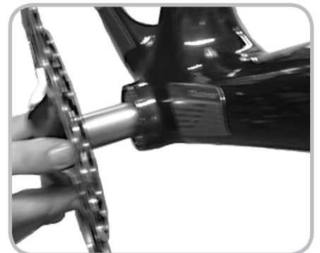
Figure 14.21. Sliding the axle through the bearings
