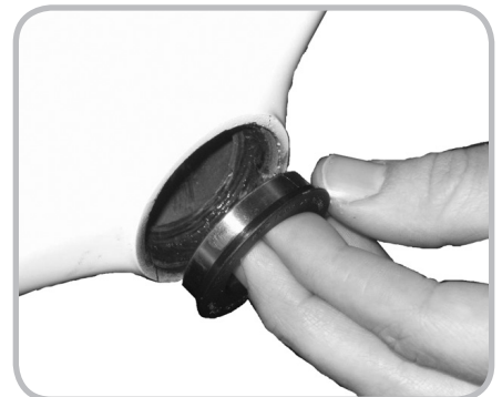
Figure 14.35. Pressing the bearing into the frame with the shield on the outside
