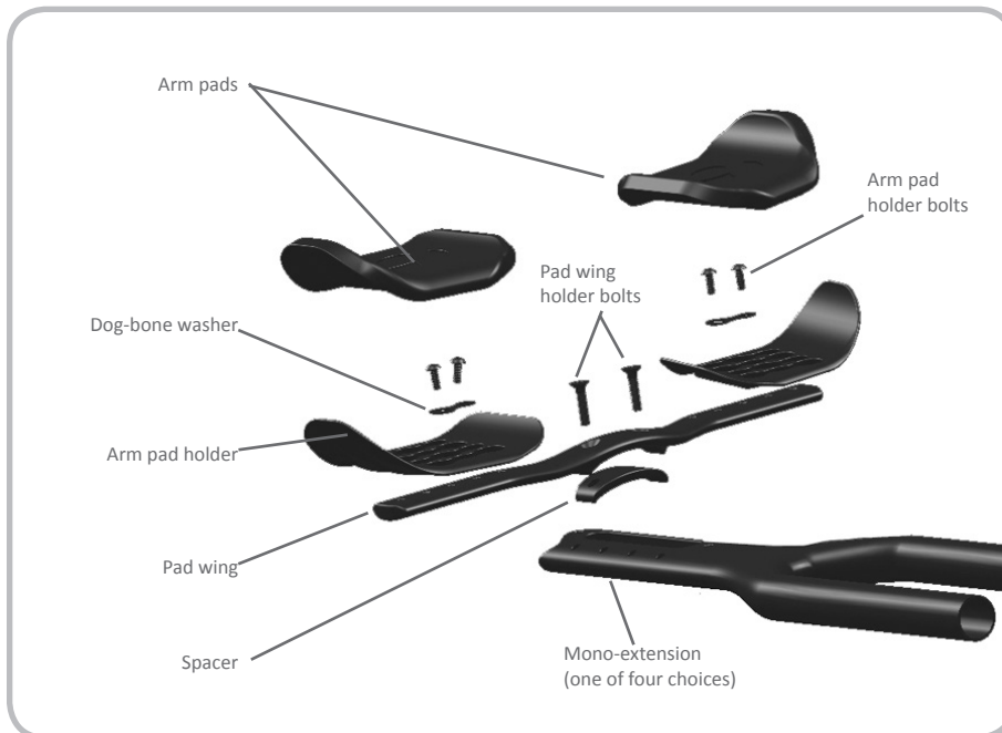
Figure 8.1. Arm supports
