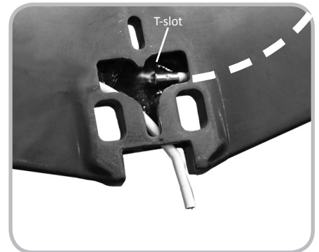
Figure 7.13. T-slot and housing routes through aerobar (bottom view of aerobar)
