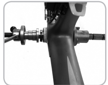
Figure 14.9. Pressing the bearing into the frame
